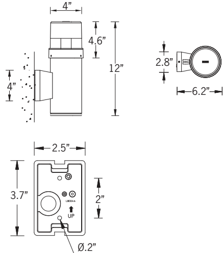
Mounting Detail
